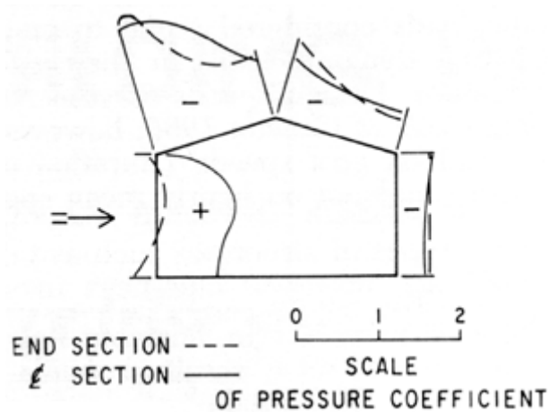
Figure 3. Distribution of pressures (+) and suction (-) on house with a low-sloped roof with wind perpendicular to eave.
