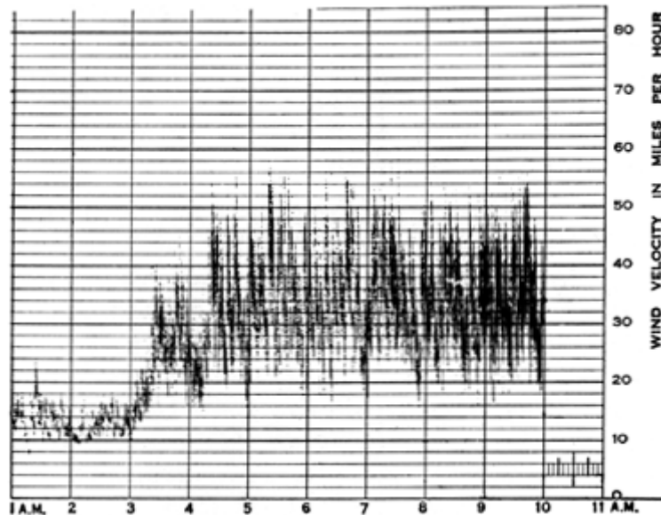
Figure 2. Typical pressure tube anemometer record
