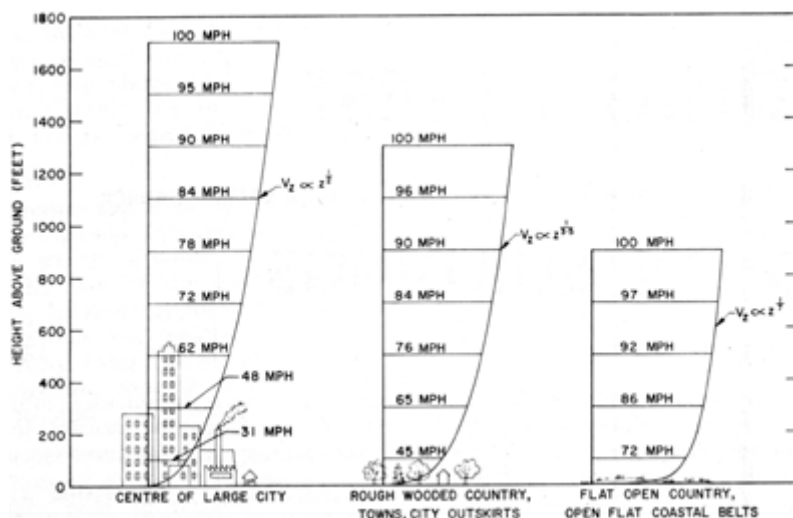
Figure 1. Mean velocity profiles over terrain with three different roughness characteristics for gradient wind of 100 mph
